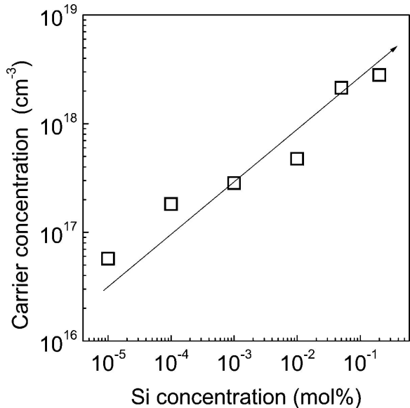
FIG. 2. Free-carrier concentration as a function of the nominal \text{Si}_{\text{con}} . The arrow indicates a systematical increase.
