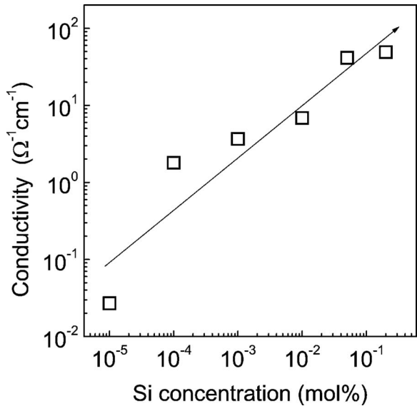
FIG. 1. Electrical conductivity as a function of the nominal \text{Si}_{\text{con}} . The arrow indicates a systematical increase.
